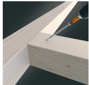
Connection of main and auxiliary beams
